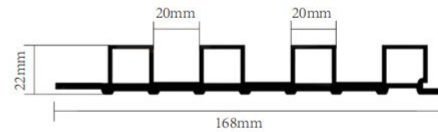
Name: 168 Hollow fluted wall panel
