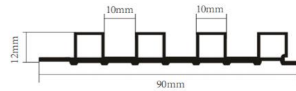
Name: 90 Hollow fluted wall panel
