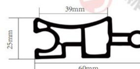
Name: 60 rotating grille panel
