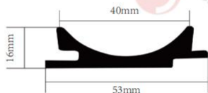
Name: 40 Inner arc solid grille
